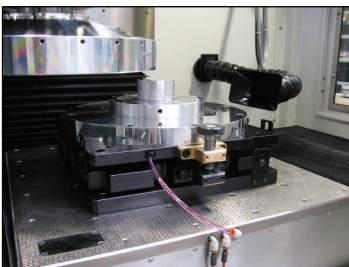
Shown above with optional air bearing A-axis and manual tip/tilt stage
