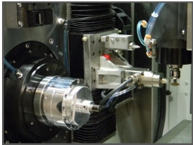
CNC Wheel Dressing System
